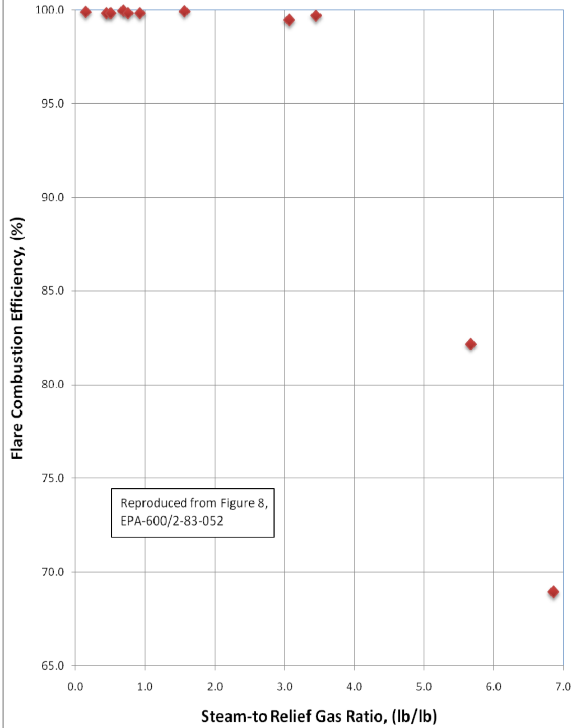
Figure 1 Effect of Steam-to Relief Gas Ratios on Flare Combustion Efficiencies
